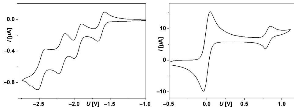
Figure 9. Cyclic voltammograms of RuL2 (1 mM) in CH 3 CN containing Bu 4 NBF 4 (0.1 M) vs. Fc/Fc + at 0.0 V (scan rate 0.05 V s -1 , step potential 0.01 V).
