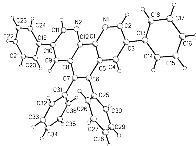
Figure 4. Solid-state structure of L2.
