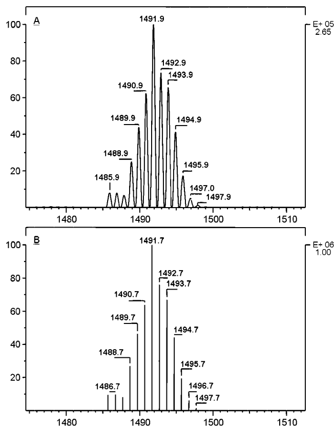
Figure 6. [\text{RuL4} - \text{PF}_6]^+ peak of the ESI-MS of RuL4 in MeOH (A) and the corresponding isotopic pattern (B) of \text{C}_{88}\text{H}_{104}\text{N}_6\text{RuPF}_6 .
