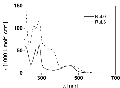
Figure 8. Absorption spectra of RuL0 and RuL3 in CH 3 CN.
