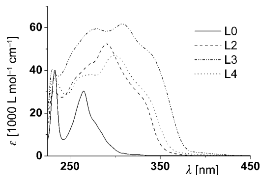
Figure 7. Absorption spectra of LR ( R = 0, 2, 3, 4 ) in \text{CH}_2\text{Cl}_2 (DCM).
