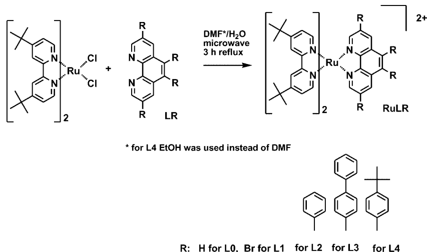
Figure 2. Naming of ruthenium complexes and corresponding ligands.
