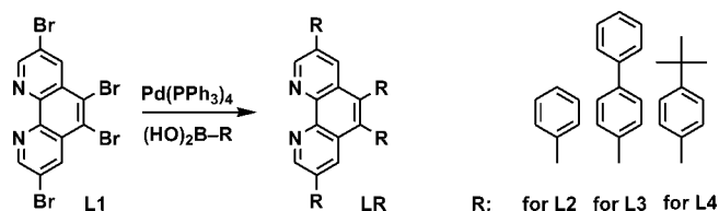
Figure 3. Synthetic route to tetraaryl-substituted phen ligands.
